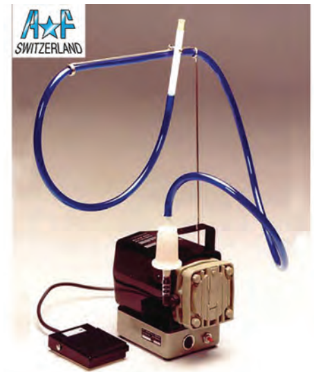
Vacuum Pump Dust Remover - A*F Swiss
